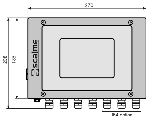
Version sans IHM - Version without HMI
